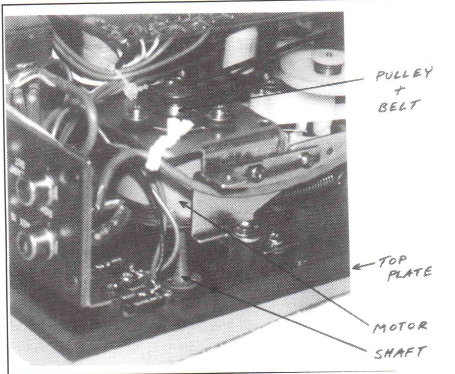
Recorder turned upside down, with the bottom case removed. The speed control shaft fits into the back of the new motor.
