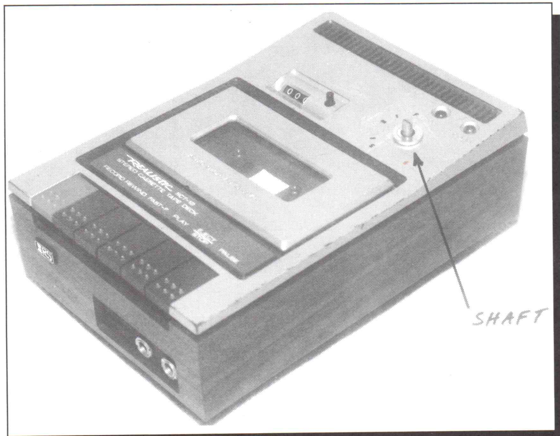
A Realistic SCT-12. The new speed control shaft is at the right, with knob removed (the washer around the shaft is optional).
